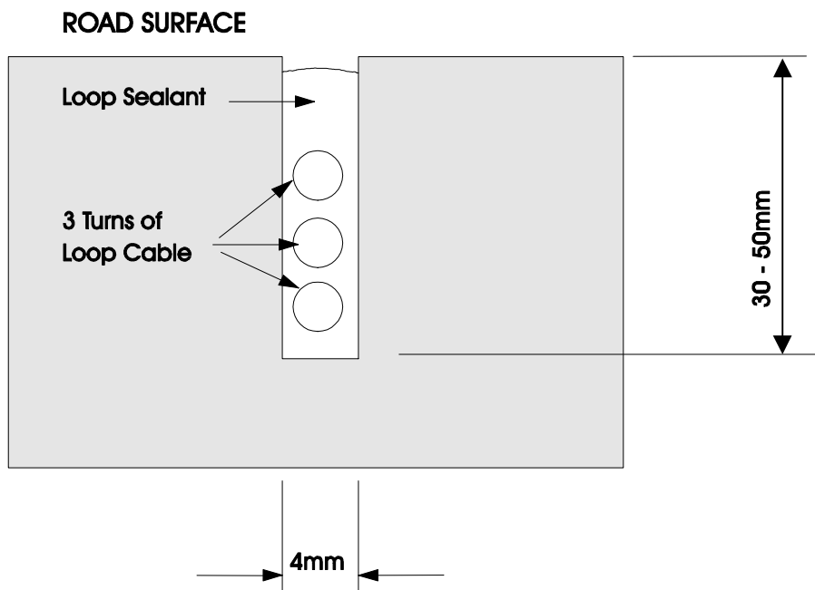
Figure 5.2 Slot Details
