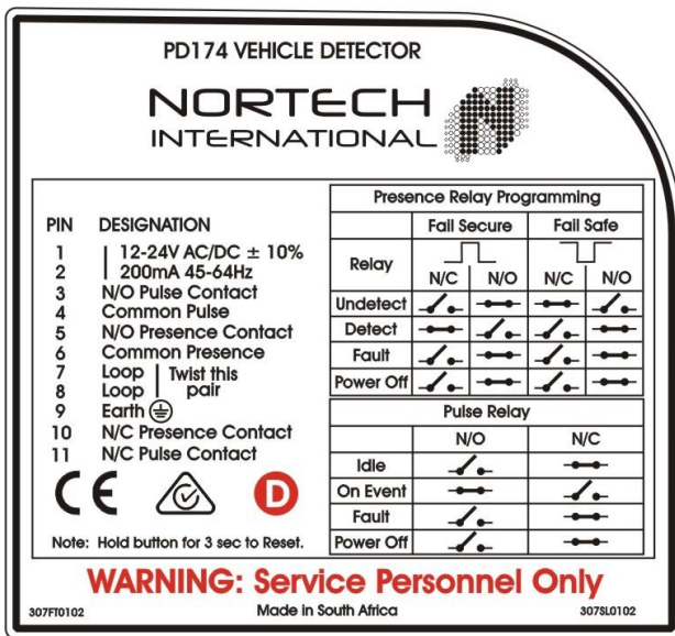
Figure 9. Example of PD17x side labels. Power supply requirements and pin connections are clearly stated on the side of the unit. 11 Pin configuration is shown on the left and DIN Rail version on the right
