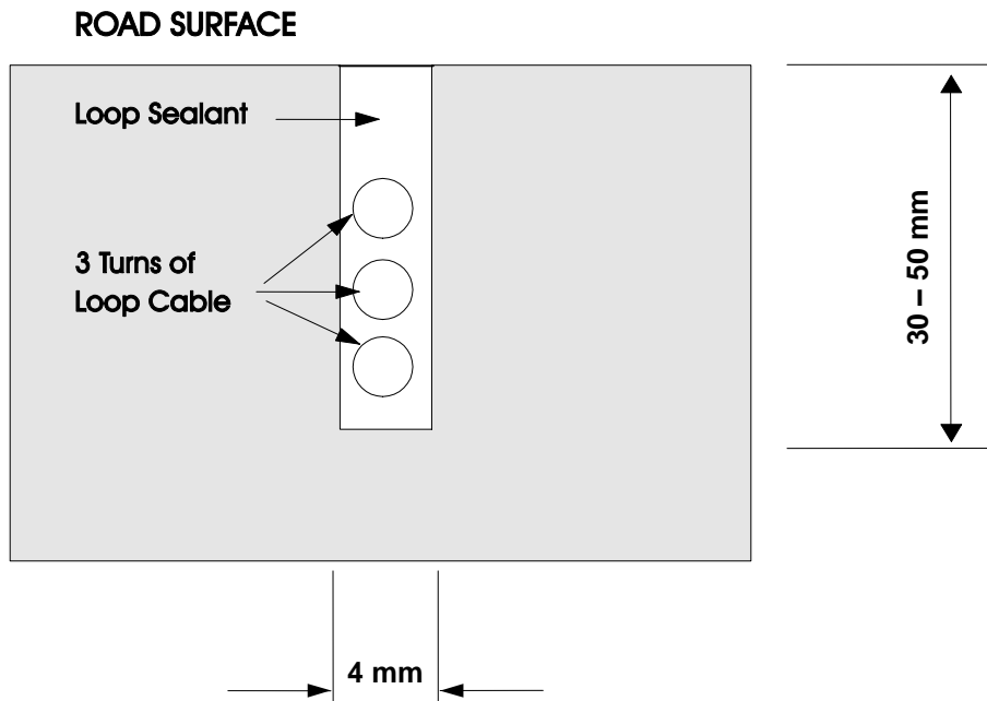
Figure 8. Slot details
