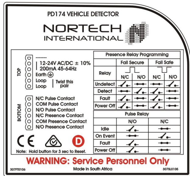
Figure 9. Example of PD17x side labels. Power supply requirements and pin connections are clearly stated on the side of the unit. 11 Pin configuration is shown on the left and DIN Rail version on the right
