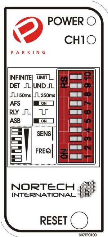
Figure 3. PD17x Faceplate
