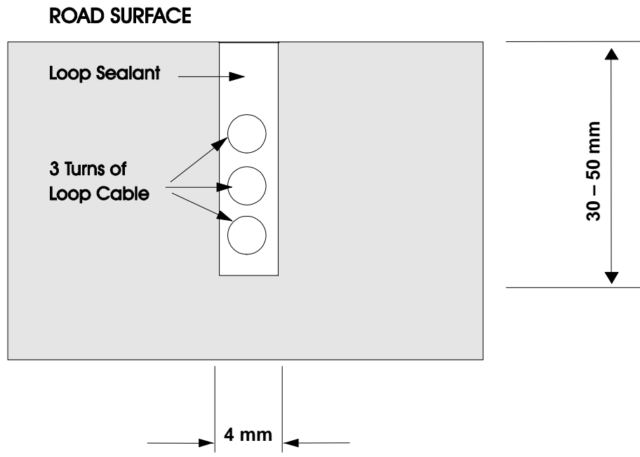
Figure 5.2 Slot details
