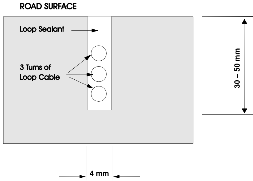
Figure 5.2 Slot details
